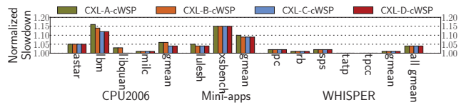
Fig. 17: Normalized slowdown of cWSP to the baseline (original program on CXL devices without crash consistency support) with varying CXL configuration; lower is better
